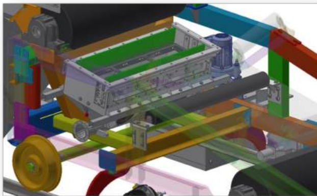
CUSTOM ULTRA-LOW PROFILE BELT WIPE
