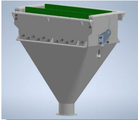
SINGLE-CONE BELT WIPE
